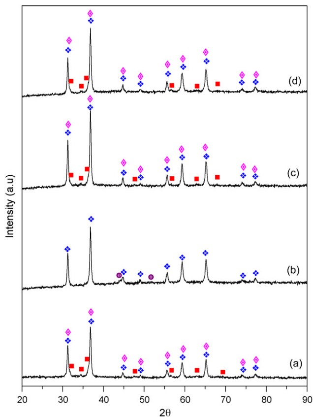
Fig. 1. Diffraction patterns of CoZA9 catalysts: (a) fresh; (b) reduced; (c) after being used at 500 °C; (d) after being used at 600 °C. \blacklozenge : \text{ZnAl}_2\text{O}_4 , \blacksquare : \text{ZnO} , \blacklozenge : \text{CoAl}_2\text{O}_4 and/or \text{Co}_3\text{O}_4 , \circ : \text{Co}^\circ .
