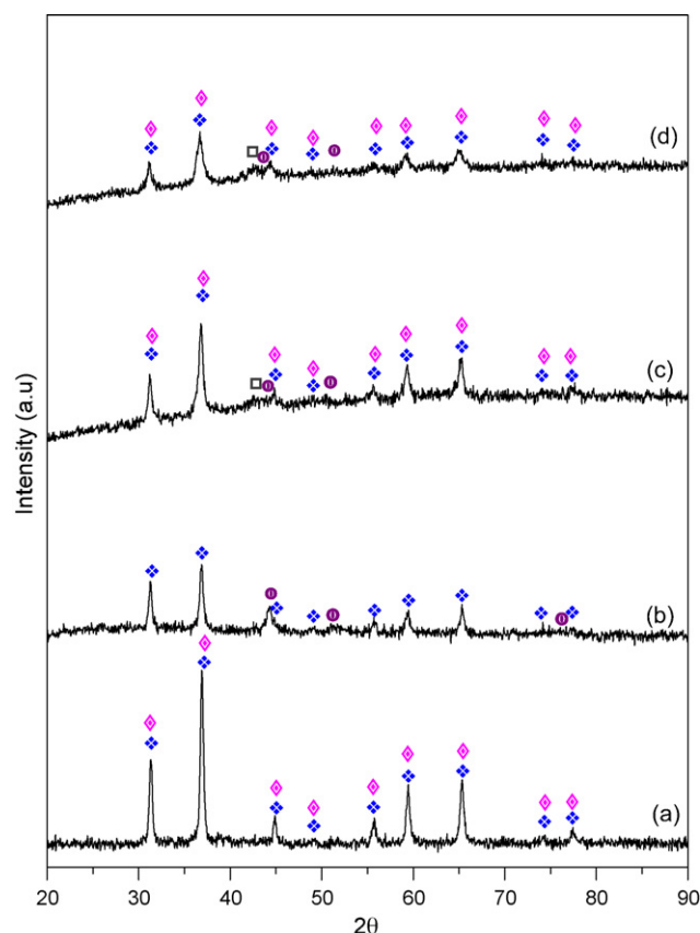
Fig. 2. Diffraction patterns of fresh CoZA25 catalysts: (a) fresh; (b) reduced; (c) after being used at 500 °C; (d) after being used at 600 °C. \blacklozenge : \text{ZnAl}_2\text{O}_4 , \blacksquare : \text{ZnO} , \blacklozenge : \text{CoAl}_2\text{O}_4 and/or \text{Co}_3\text{O}_4 , \circ : \text{Co}^\circ .
